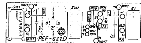
PEF-622D PCB
