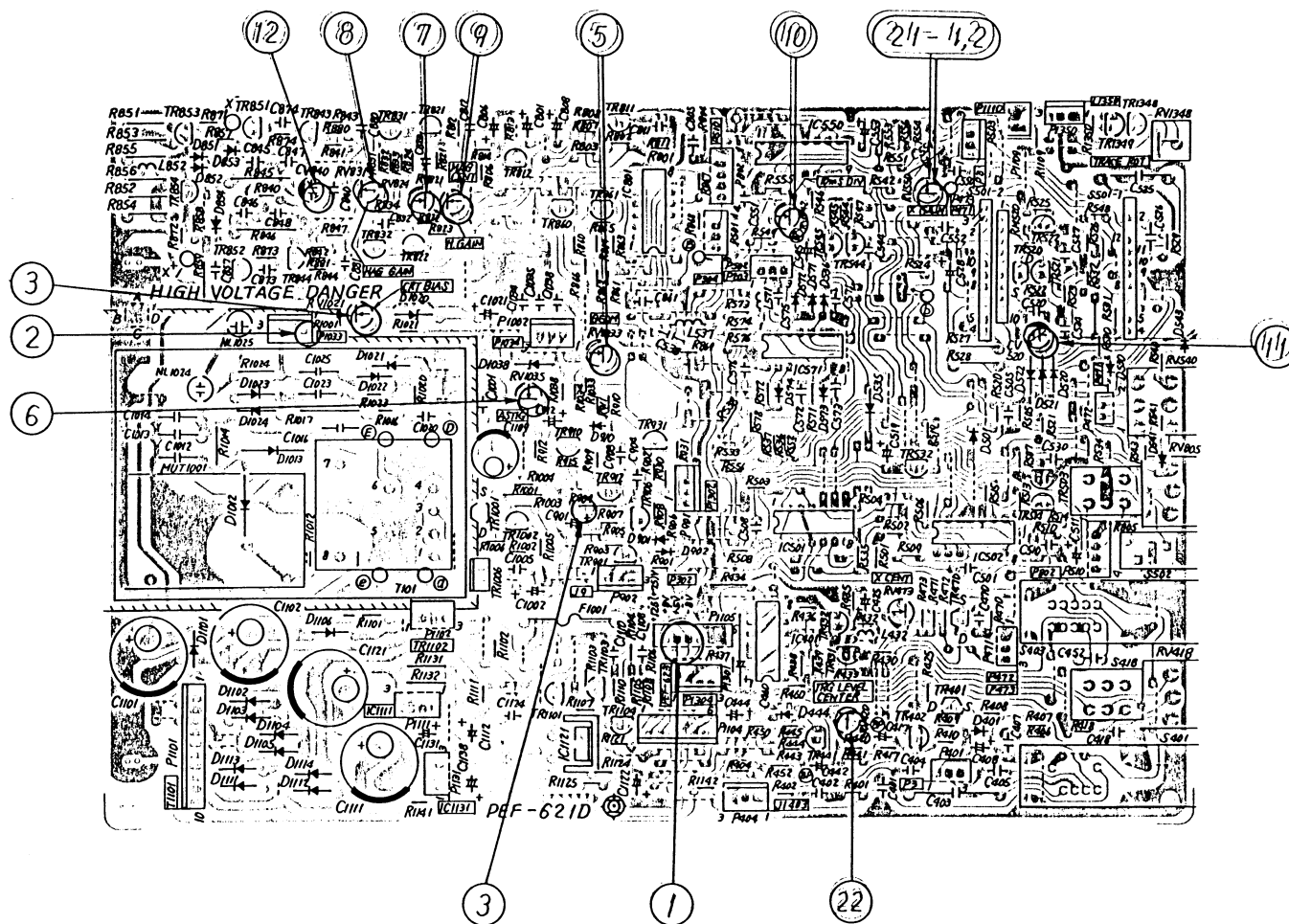
PEF-621D PCB
