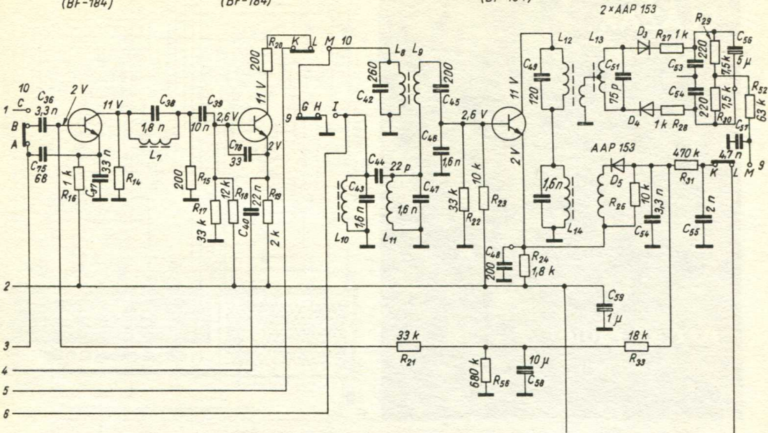
BF-194 (BF-184)
