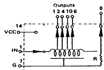
Schematic Diagram for 5 Delays Output
